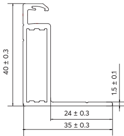
Frame profile
