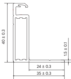
Frame profile
